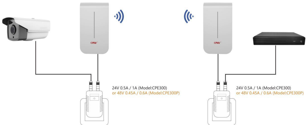
Wireless Bridge-Power Supply-Camera
